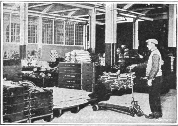
Fig. 8—Telescopic boxes on platforms are used by the Pierce-Arrow Motor Car Co., Buffalo, N. Y., in connection with Cowan elevating trucks. Box sections are of standard size and can be built up as required. Note saving of floor space made possible
